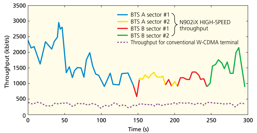
Figure 2 Changes in throughput performance over time
