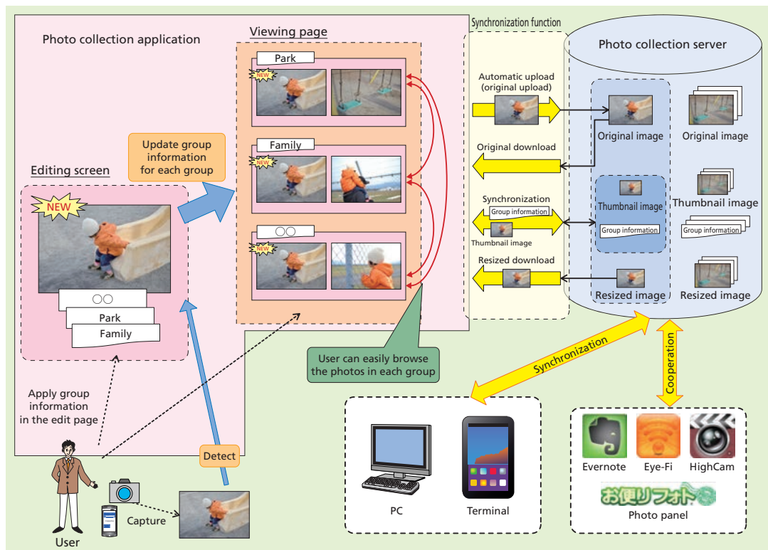
Technology Reports Android Application Development in DOCOMO Cloud (P.4) Flowchart of Photo Collection service
