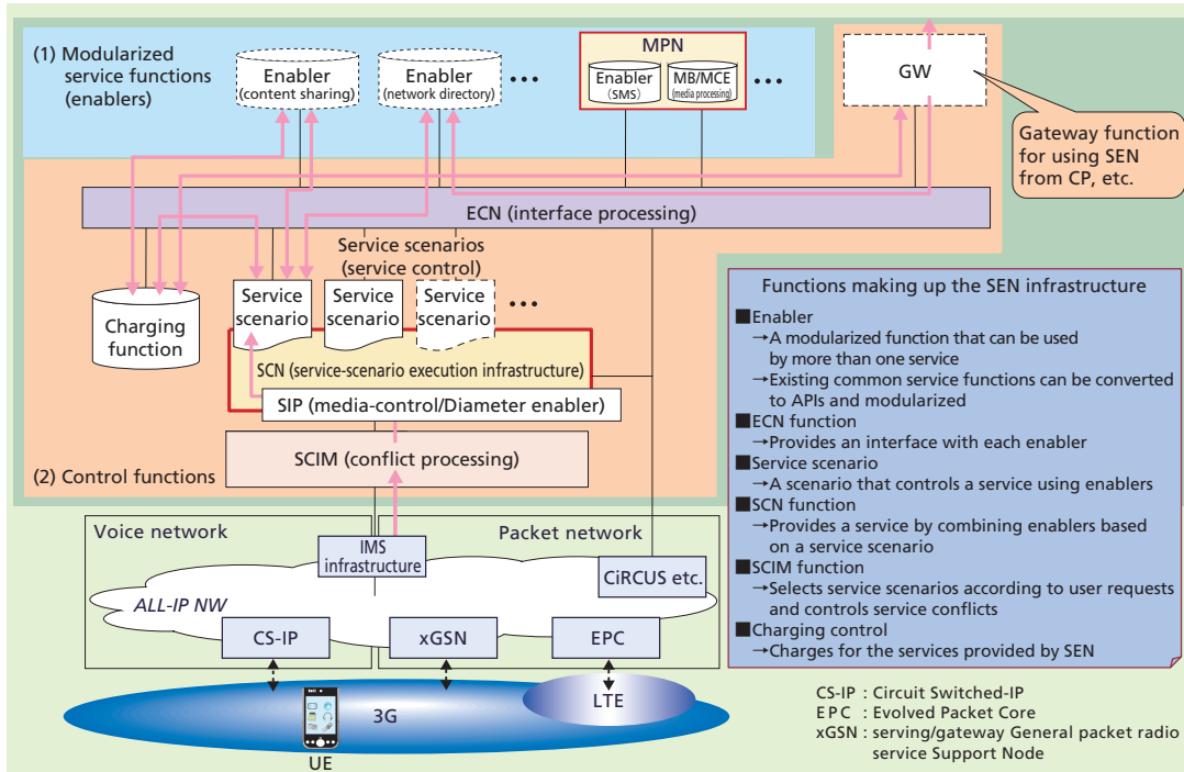
Technology Reports SEN Infrastructure for Configuring a Network Cloud (P.4) Overall logical configuration of the SEN infrastructure
