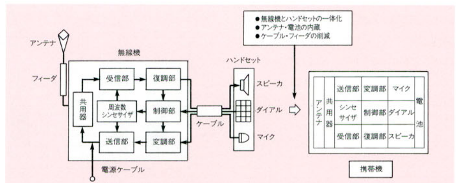
図3 移動機から携帯機へ Portable Radio Telephone Unit Design from Mobile Radio Telephone Unit
