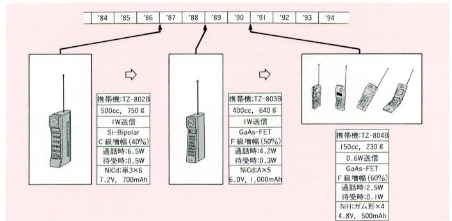
図5 携帯機の開発経緯 Figure 5 Progress of 800 MHz Portable Radio Telephone Unit
