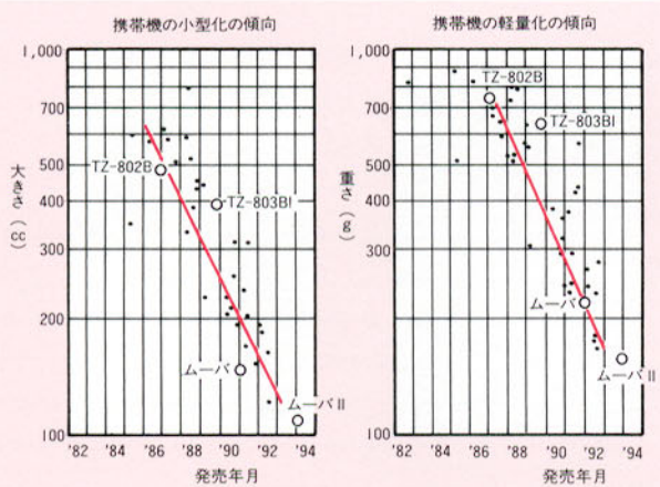
図18 携帯機の小型・軽量化の傾向 Figure 18 Trend of Size and Weight of Portable Telephone Unit
