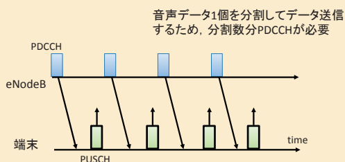
図7 segmentation
